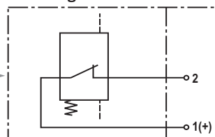
WE-1SP-EN175301-803
