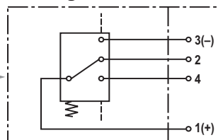
WE-1SP-M12x1
